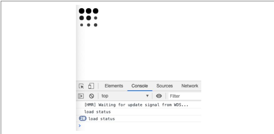
Figure 9-12. Suspend recursion
